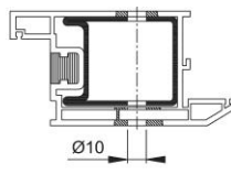
PVC profile
