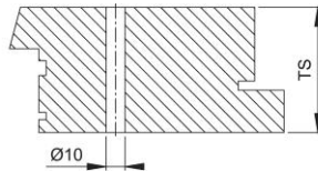
houten-profiel
